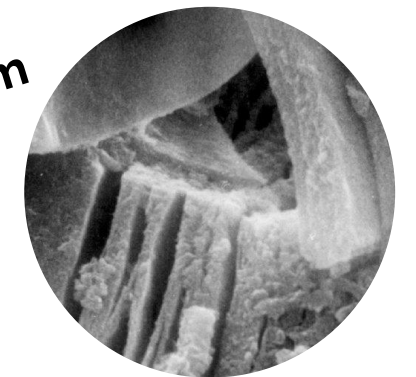
Clay mineral
